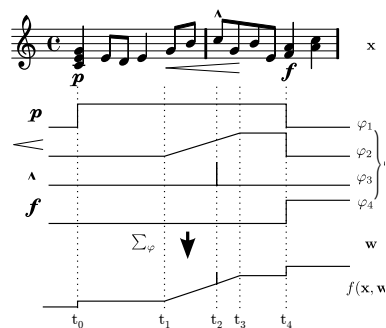
Fig. 1. Schematic view of note intensities as a weighted sum f(\mathbf{x}, \mathbf{w}) of basis functions \varphi , representing dynamic annotations
