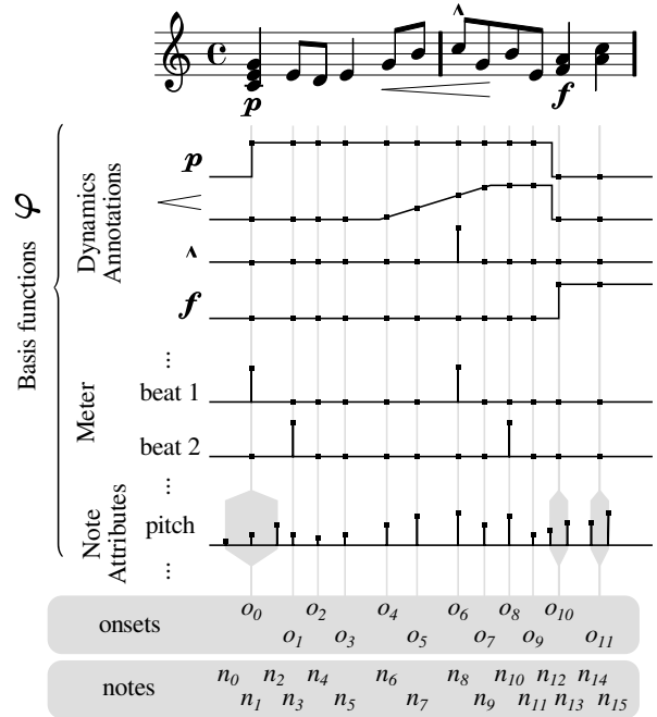
Figure 1. An example of basis functions modeling of dynamic annotations, meter and pitch.
