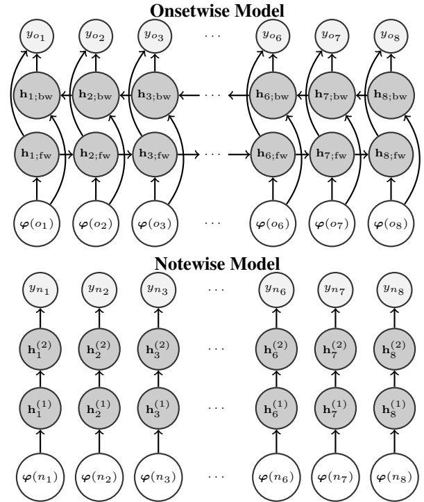
Figure 1. Neural architectures used for the BM models.
